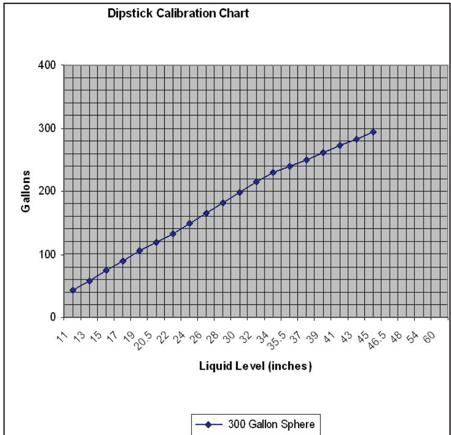
300 Gallon Fully Plumbed Pump Tank
